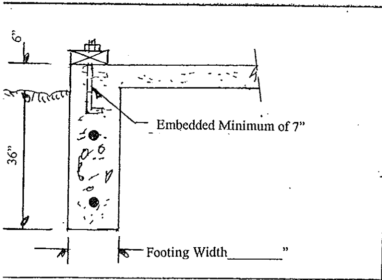
FROST FREE FOOTING (Required for Bldgs over 400 Sq. Ft.)
