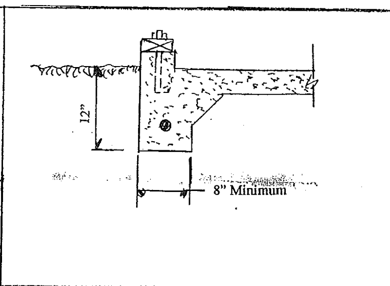
MONOLITHIC SLAB (Optional for Bldgs up to 400 Sq Ft)
